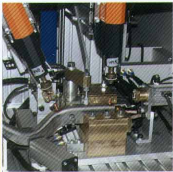
Dual head facility enables simultaneous welding of studs
