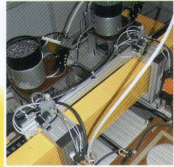
Two head automatic stud feed system with bowl feed
